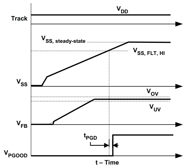
Figure 32. PGOOD Signal
