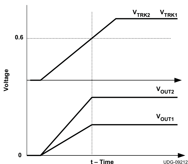
Figure 27. Ratiometric Voltage-Tracking Schematic Figure 28. Ratiometric Voltage-Tracking Waveform
