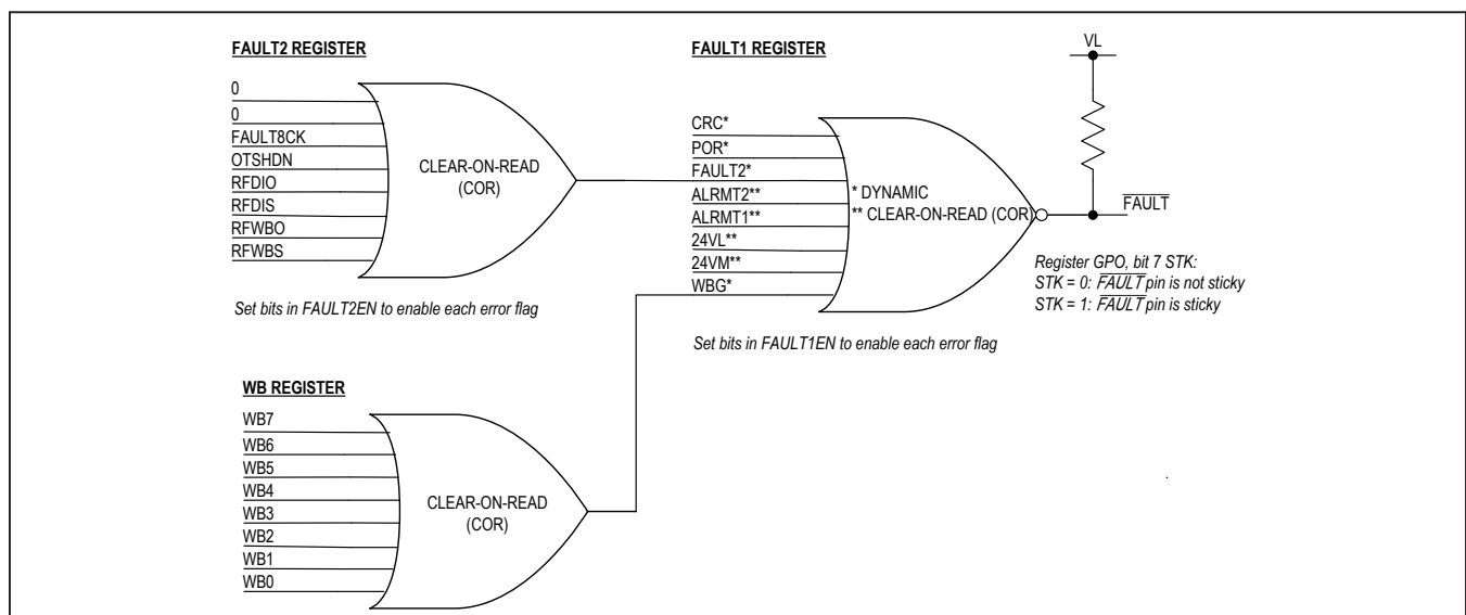
Figure 8. \overline{\text{FAULT}} Output Sources
