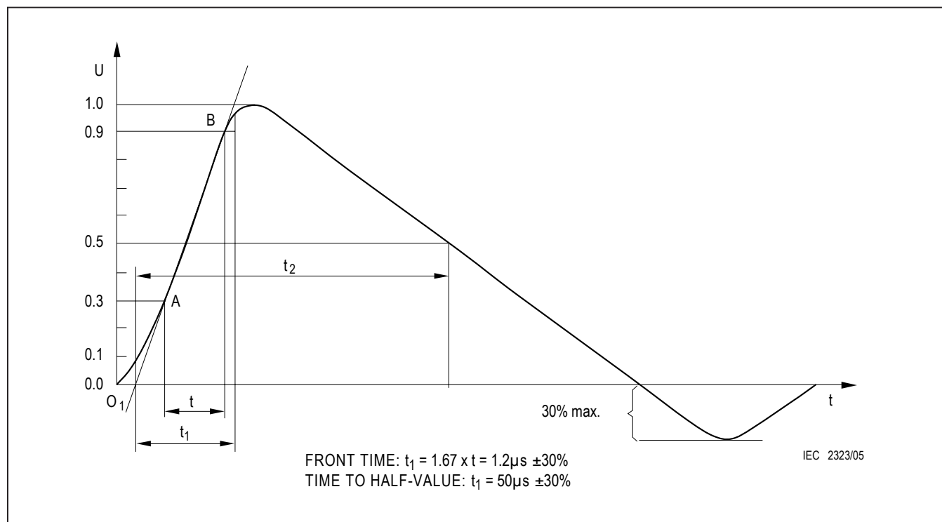
Figure 15. 1.2/50 \mu s Surge Voltage Waveform
