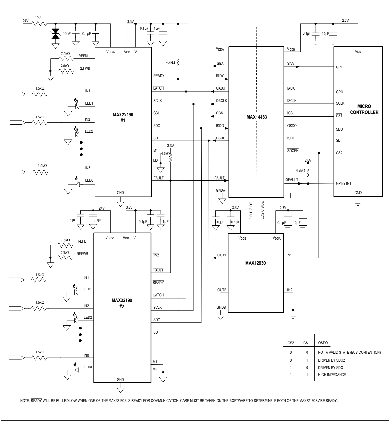
Figure 10. 16 Input, Independent Slave SPI (Separate \overline{\text{CS}} for Each SPI Slave)
