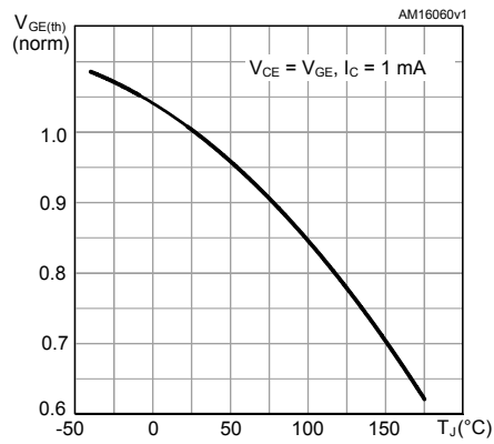
Figure 13. Normalized V_{GE(th)} vs junction temperature
