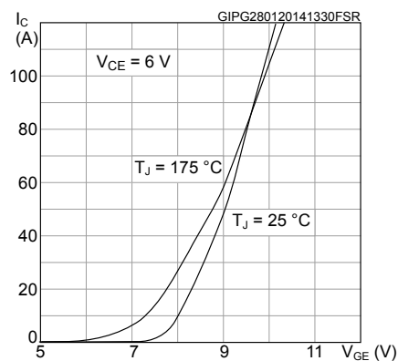
Figure 3. Transfer characteristics
