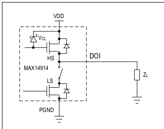
Figure 4. Digital Output Driver
