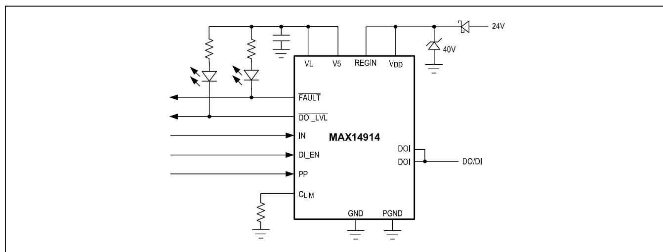
Figure 6. DO/DI Configuration with External Schottky Diode
