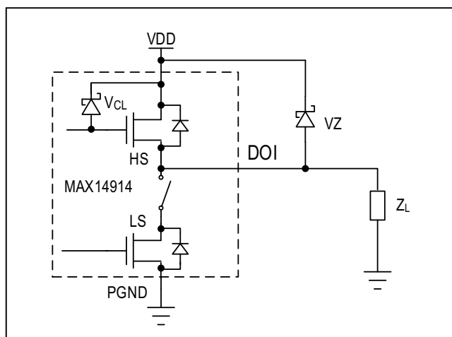
Figure 5. External Inductive Load Clamping
