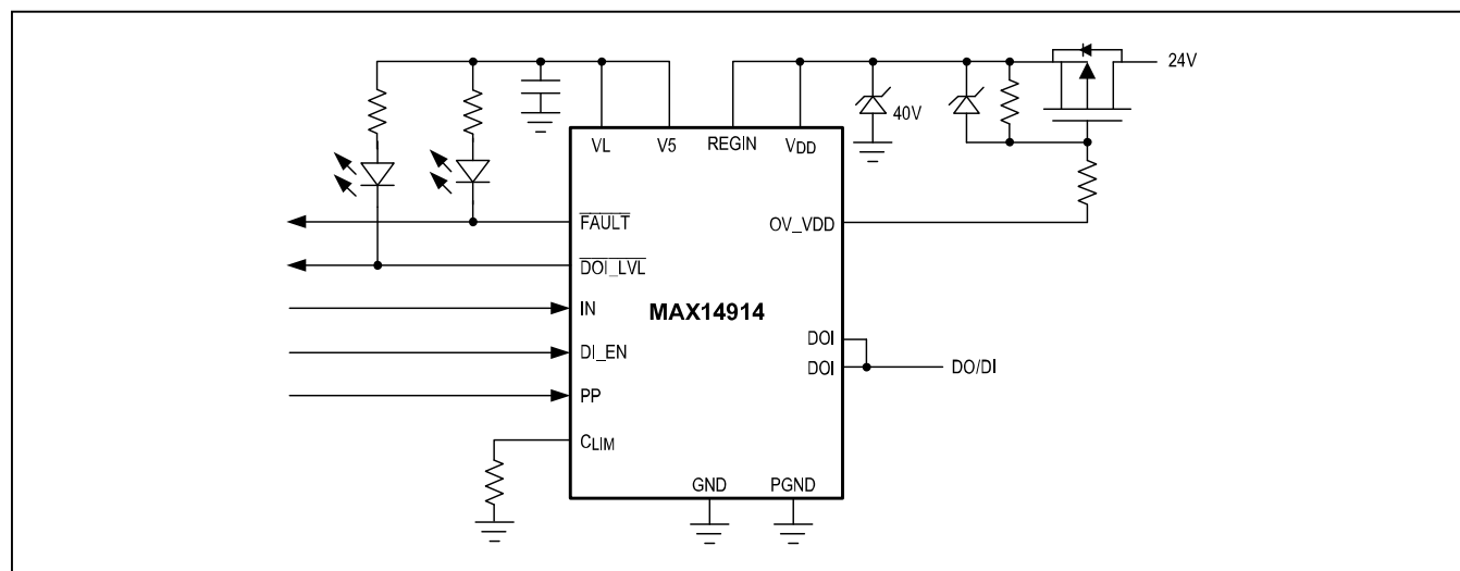
Figure 7. DO/DI Configuration with External pMOSFET
