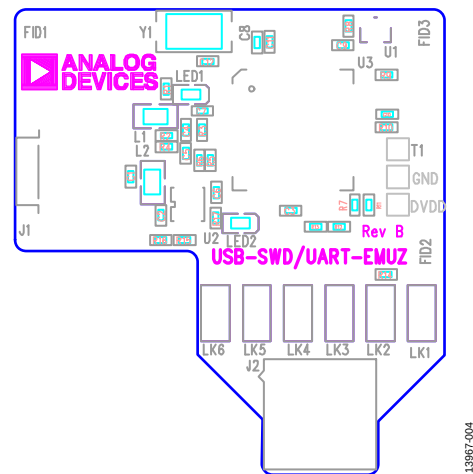
Figure 8. Emulator, Top View
