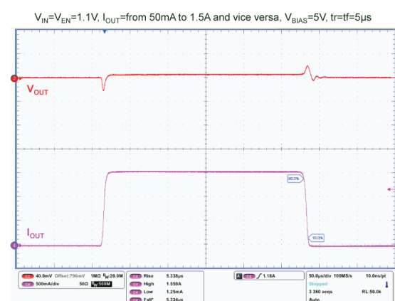
Figure 17. Load transient
