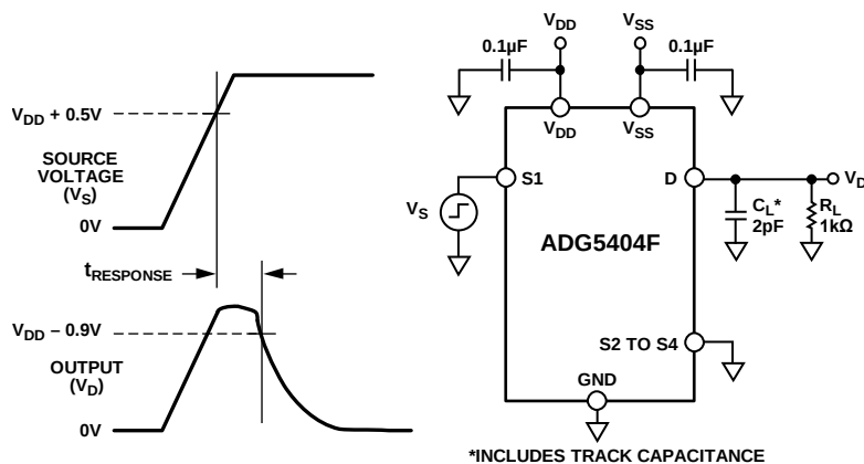
Figure 40. Overvoltage Response Time, t_{\text{RESPONSE}}
