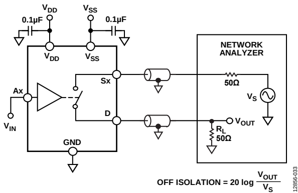
Figure 34. Off Isolation
