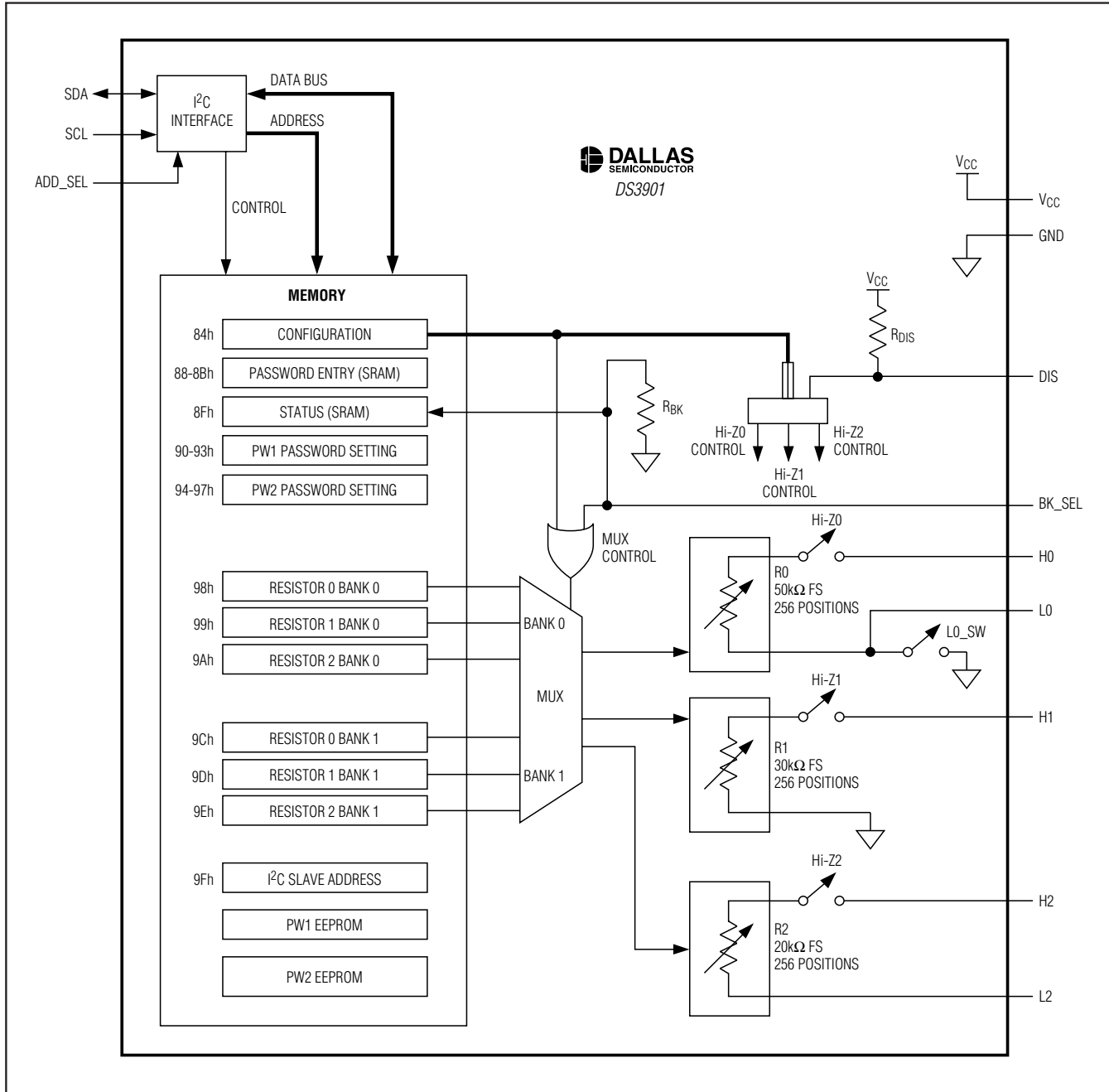
Block Diagram
