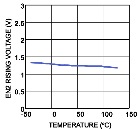
EN2 Rising Voltage
