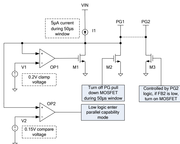
Figure 3: PG Functional Schematic
