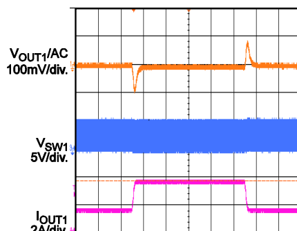
CH1 Transient
