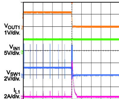
CH1 Short Enter
