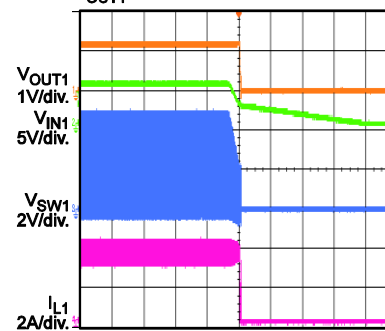
VIN Power Down with 3.5A Load (CH1)
