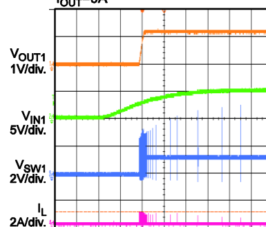
VIN Power Up without Load (CH1)
