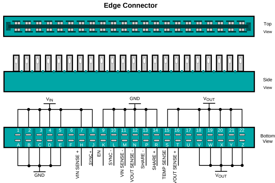
Figure 3. Edge Connector Diagram
