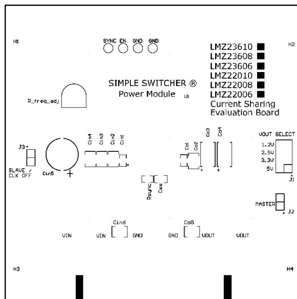
Figure 12. Top Silkscreen
