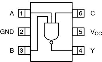
Figure 2. SC70 (Top View)
