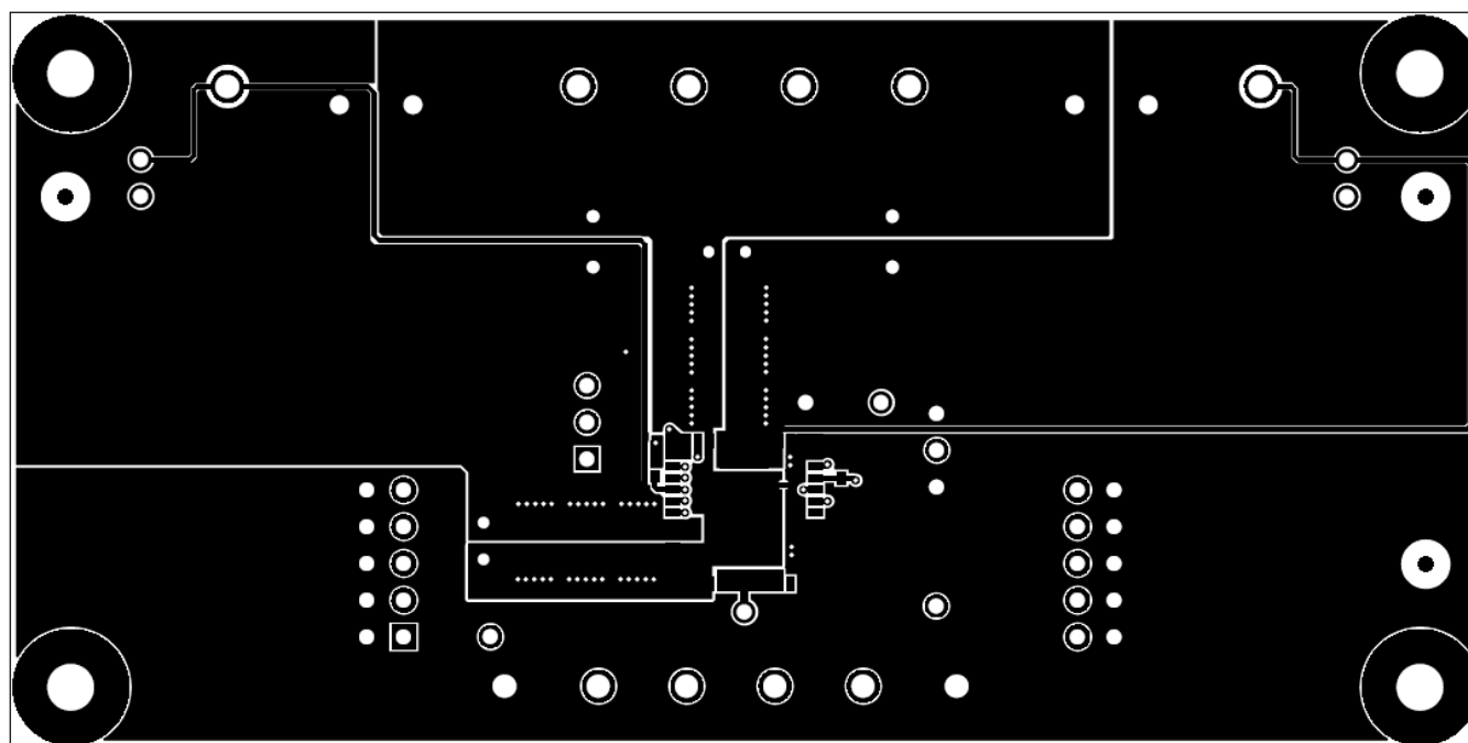
Figure 12. LMZ34202EVM Layer 1 Copper
