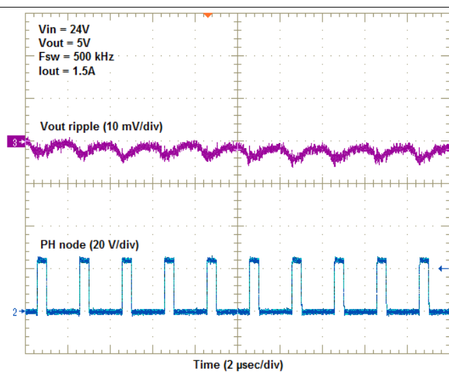
Figure 5. LMZ34202EVM Ripple Voltage (Fsw = 500 KHz)
