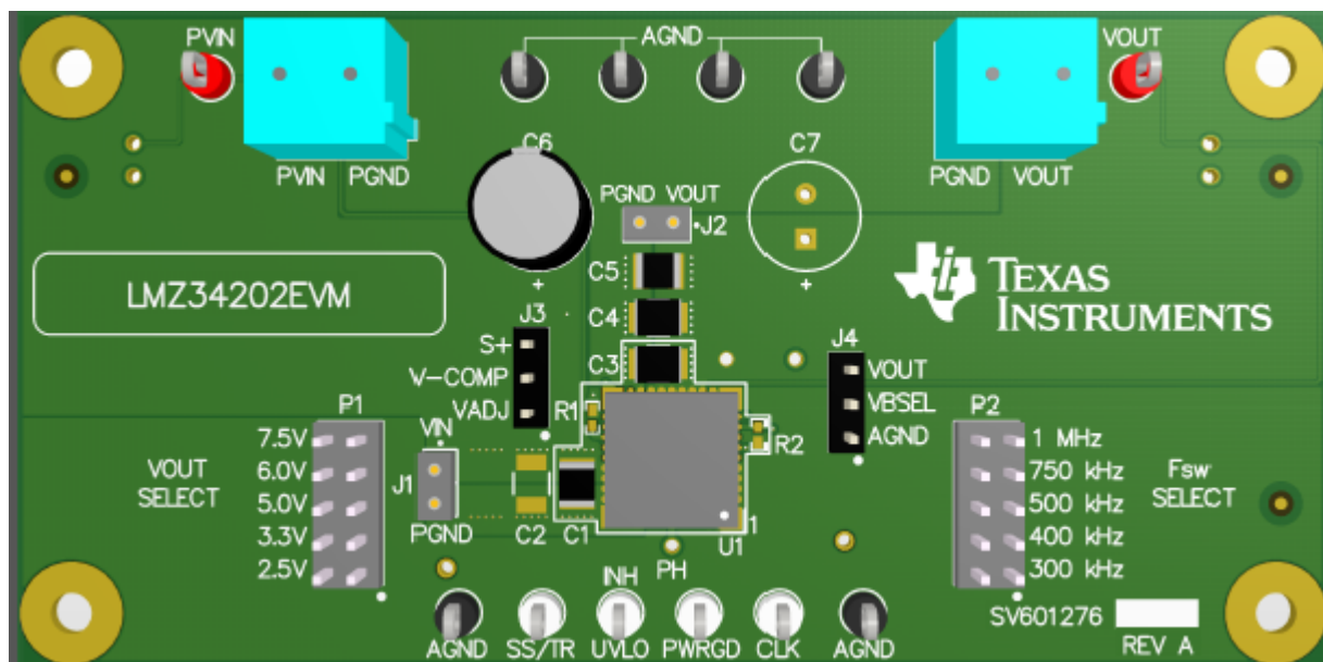
Figure 1. LMZ34202EVM User Interface
