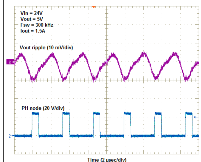
Figure 4. LMZ34202EVM Ripple Voltage (Fsw = 300 KHz)
