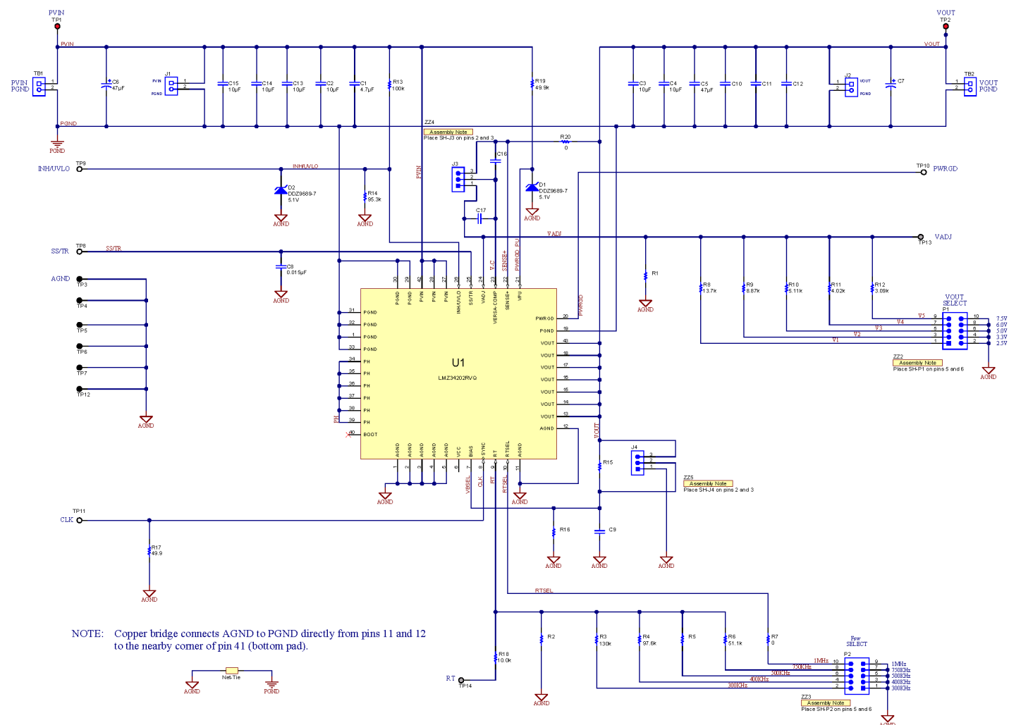
Figure 8. LMZ34202EVM Schematic
