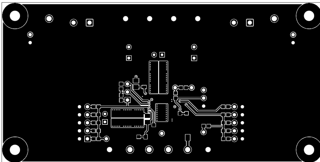
Figure 15. LMZ34202EVM Bottom-Side Copper
