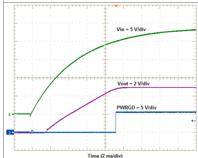
Figure 6. LMZ34202EVM Start-up Waveforms
