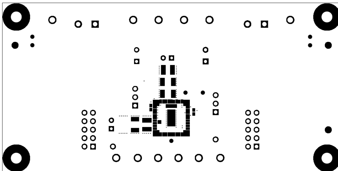
Figure 11. LMZ34202EVM Topside Soldermask
