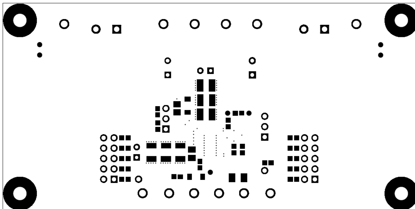
Figure 16. LMZ34202EVM Bottom Solder Mask
