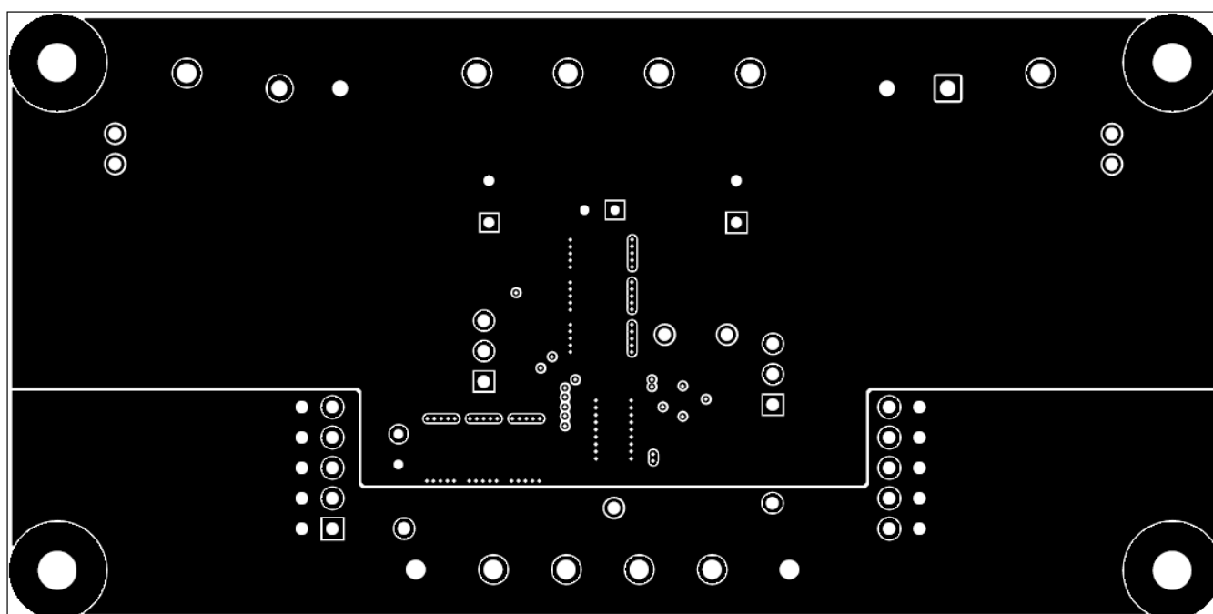
Figure 13. LMZ34202EVM Layer 2 Copper
