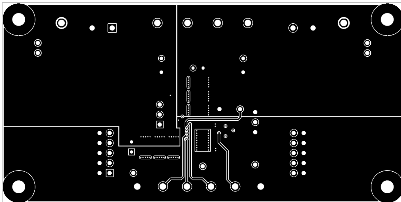
Figure 14. LMZ34202EVM Layer 3 Copper
