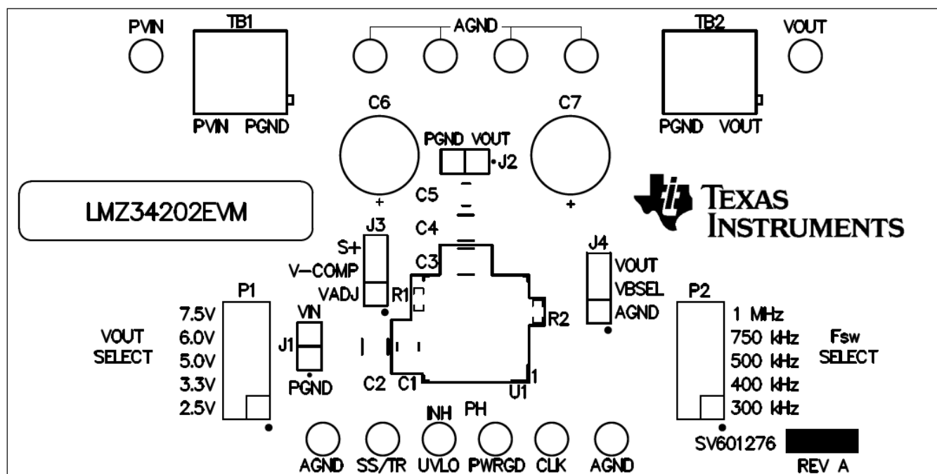
Figure 10. LMZ34202EVM Topside Component Layout
