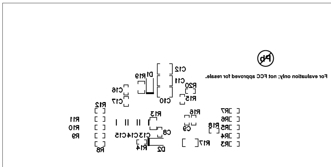
Figure 17. LMZ34202EVM Bottom-Side Component Layout
