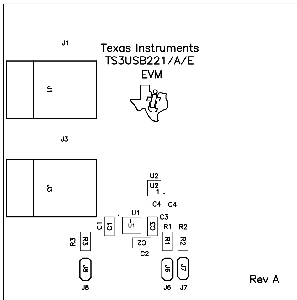
Figure 5. Top Silkscreen/Assembly
