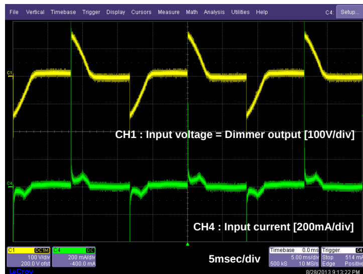
Figure11. Dimming operation waveform at phase angle=60degree
