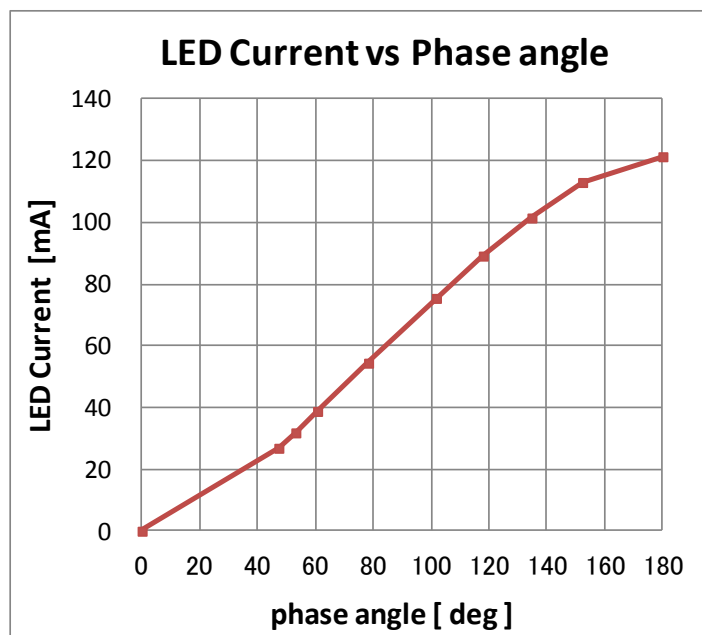
Figure8. LED current vs Phase angle
