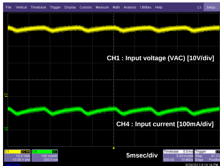
Figure7. Output waveform
