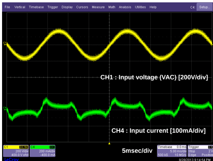
Figure6. Input waveform
