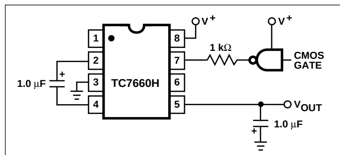
Figure 6. External Clocking
