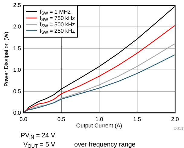
Figure 10. Power Dissipation vs Output Current
