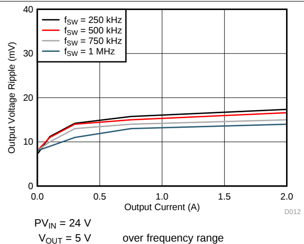
Figure 12. Voltage Ripple vs Output Current
