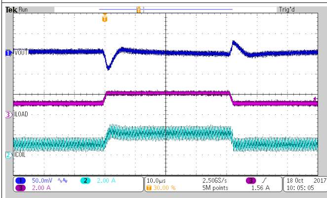
Figure 46. Load Transient Response, 1A to 2A, TPS62822
