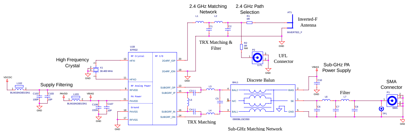
Figure 4.1. Schematic of the RF Section of the BRD4158A
