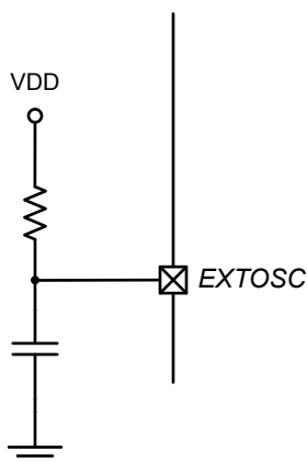
Figure 8.2. External RC Oscillator Configuration
