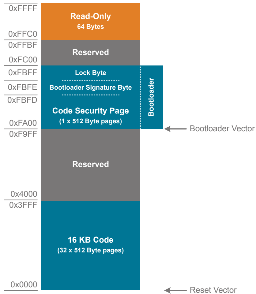
Figure 4.6. Bootloader Flash Memory Map — 16 KB Devices
