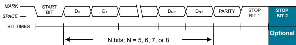
Figure 23.3. UART1 Timing With Parity
