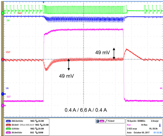
Figure 34. Transient Load 0.4 to 6.6 A – Auto Mode, V_{IN} = 3.3\text{ V} – V_{OUT} = 1.0\text{ V} – L = 0.24\text{ }\mu\text{H} – C_{OUT} = 4\text{ x }47\text{ }\mu\text{F}
