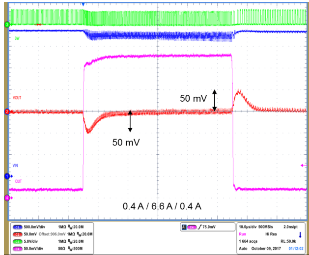
Figure 35. Transient Load 0.4 to 6.6 A – Forced PPWM, V_{IN} = 3.3\text{ V} – V_{OUT} = 1.0\text{ V} – L = 0.24\text{ }\mu\text{H} – C_{OUT} = 4\text{ x }47\text{ }\mu\text{F}
