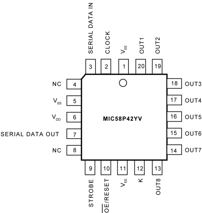
20-pin PLCC (V) (Top View)
