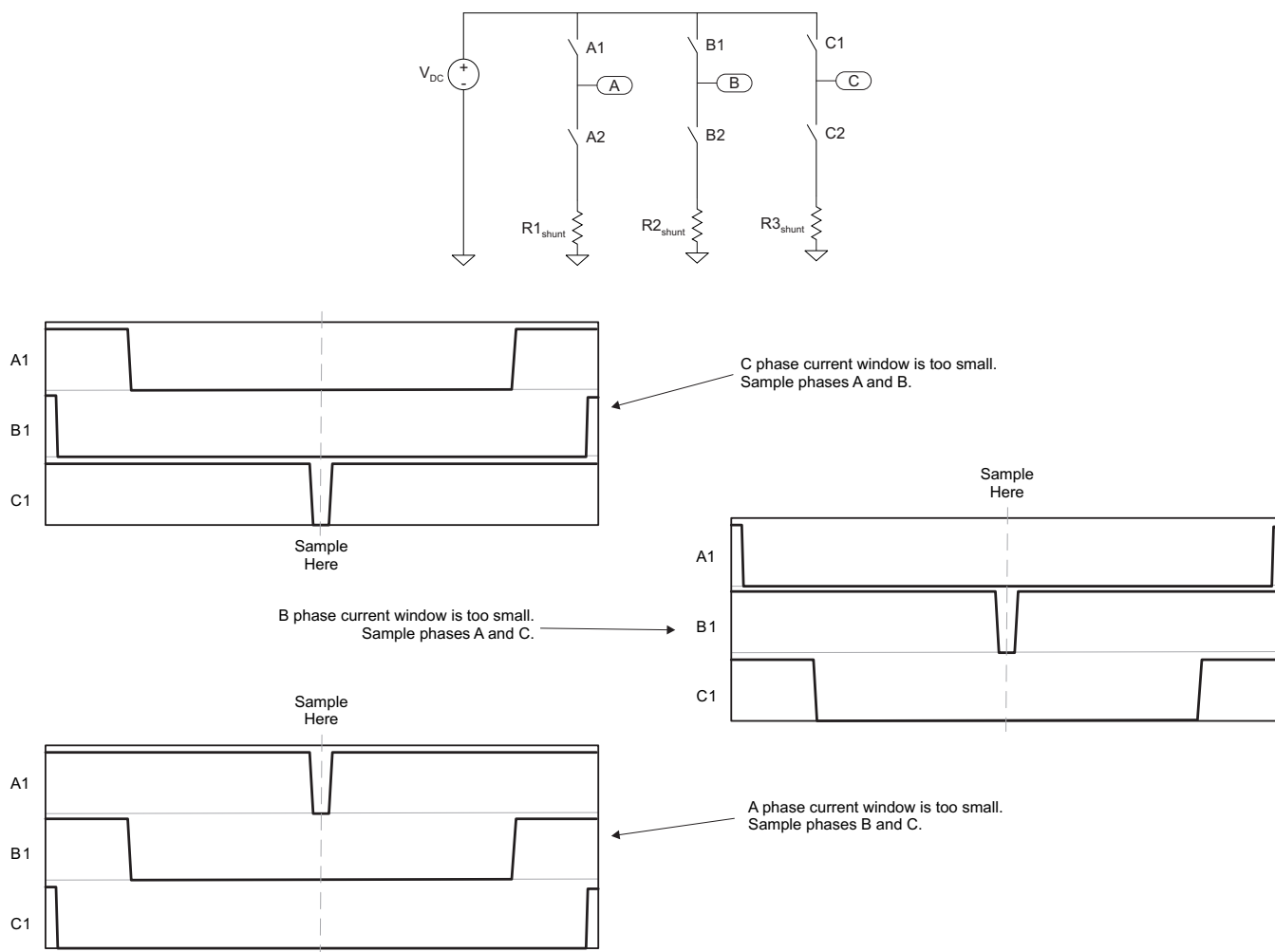
Figure 5. Inverter Using the 3-Shunt Current Sampling Technique
