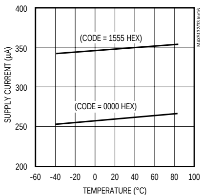
MAX5133 SUPPLY CURRENT vs. TEMPERATURE
