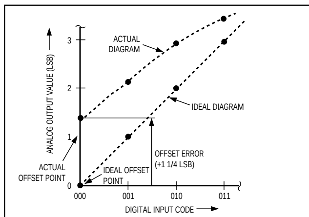
Figure 8c. Offset Error
