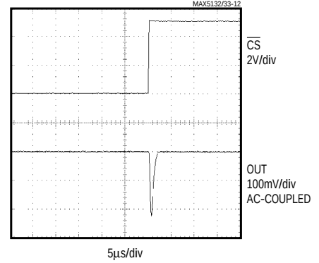
MAX5132 MAJOR CARRY TRANSITION
