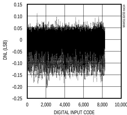
MAX5133 DIFFERENTIAL NONLINEARITY vs. DIGITAL INPUT CODE
