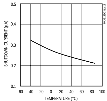
MAX5133 SHUTDOWN CURRENT vs. TEMPERATURE
