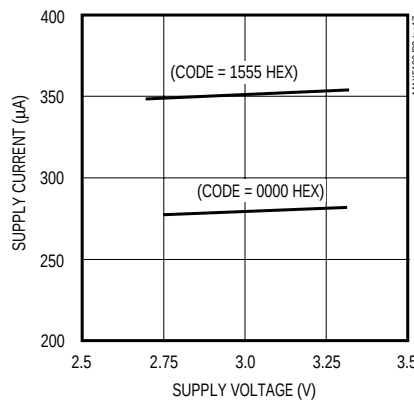
MAX5133 SUPPLY CURRENT vs. SUPPLY VOLTAGE
