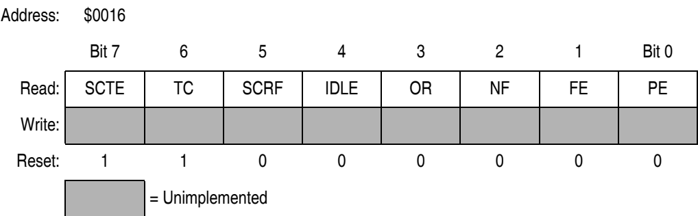
Figure 13-15. SCI Status Register 1 (SCS1)
