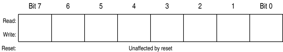
Figure 6-2. Accumulator (A)
