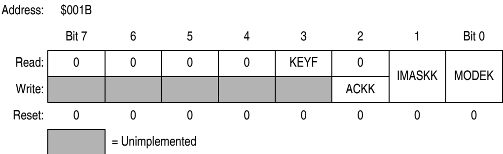
Figure 19-3. Keyboard Status and Control Register (KBSCR)
