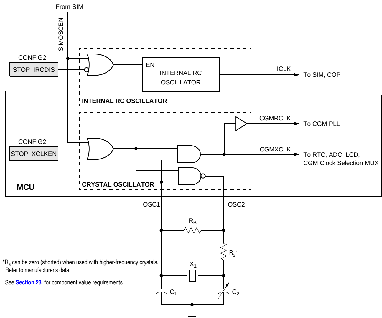
Figure 7-1. Oscillator Module Block Diagram
