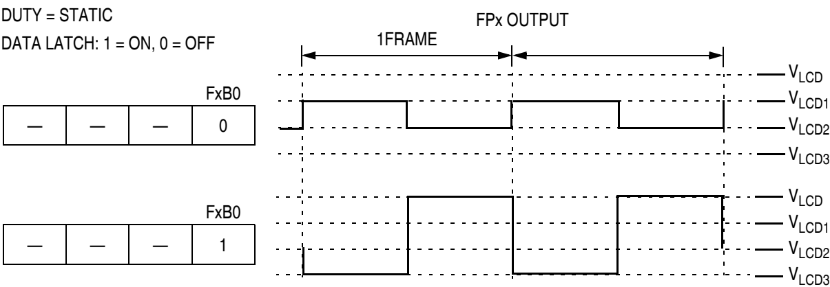
Figure 16-8. Static LCD Frontplane Driver Waveforms
