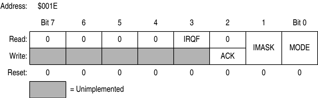
Figure 18-2. IRQ Status and Control Register (INTSCR)
