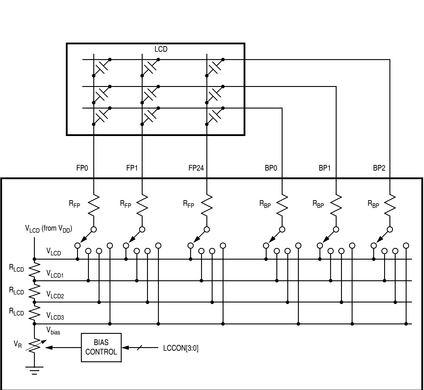
Figure 16-3. Simplified LCD Schematic (1/3 Duty, 1/3 Bias)
