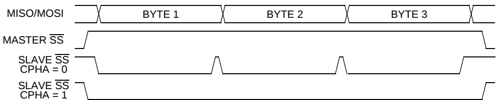
Figure 14-5. CPHA/SS Timing
