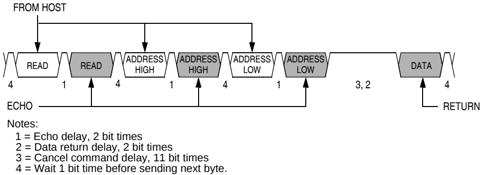
Figure 10-5. Read Transaction
