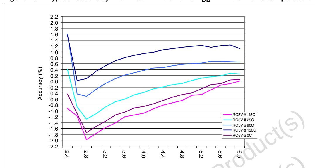
Figure 41. Typical accuracy with RCCR=RCCR1 vs V_{DD} = 2.4-6.0V and temperature
