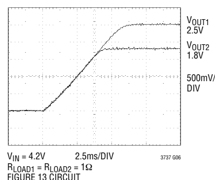
Tracking Start-Up with External Soft-Start ( C_{SS} = 10\text{nF} )
