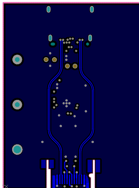
Figure 11. Bottom Layer
