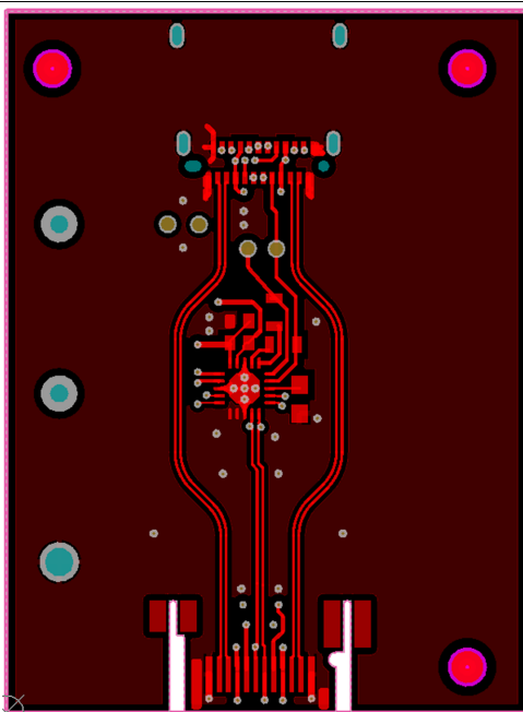
Figure 4. Top Layer
