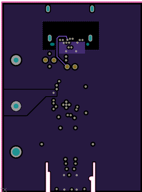
Figure 8. Power Plane 1
