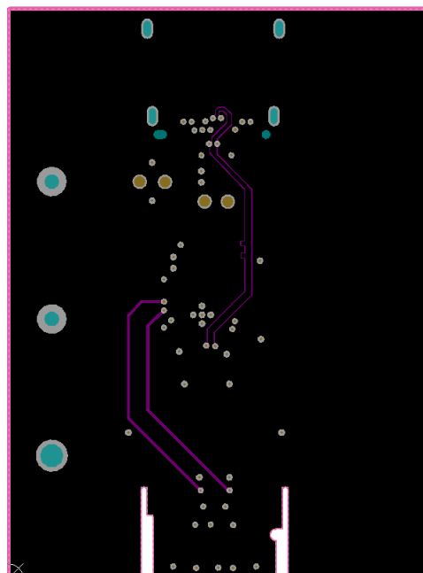
Figure 9. Ground Plane 3
