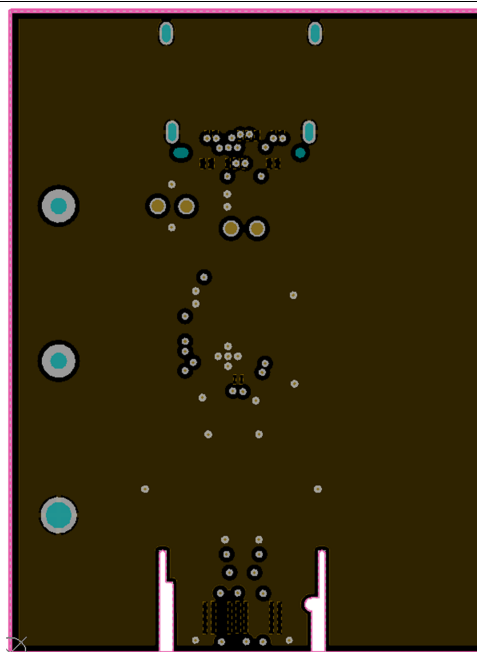
Figure 5. Ground Plane 1
