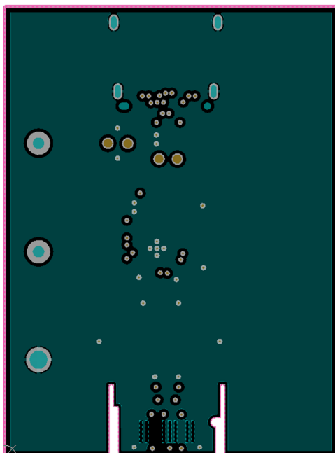
Figure 10. Ground Plane 3
