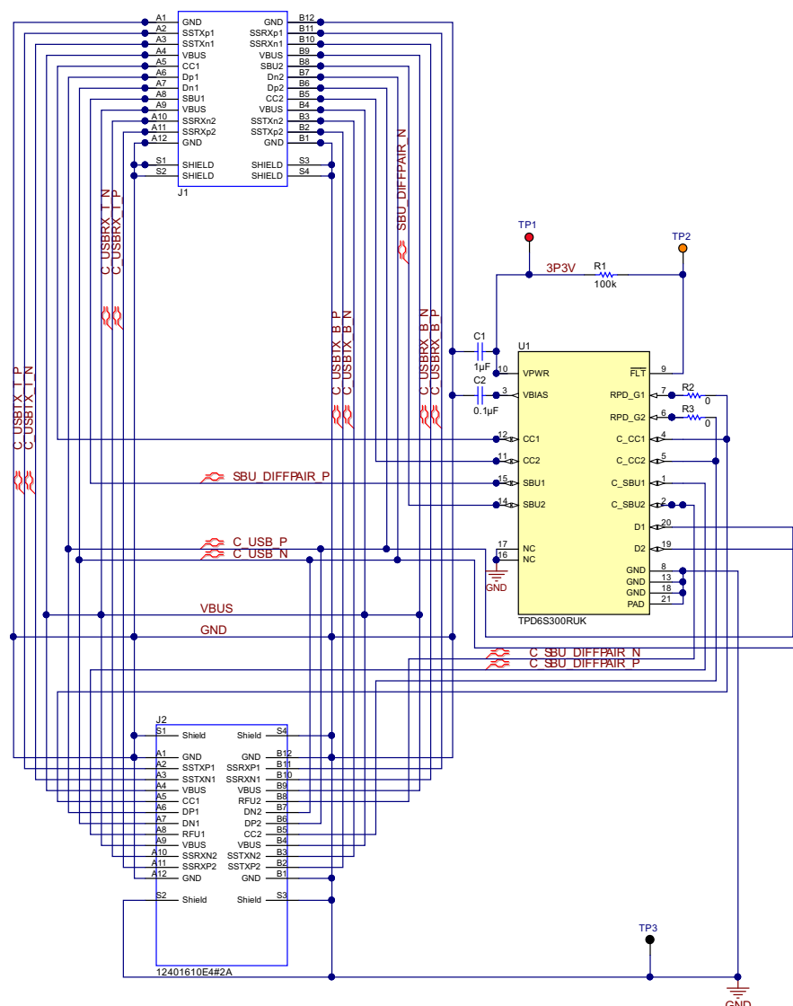
Figure 3. TPD6S300EVM Schematic
