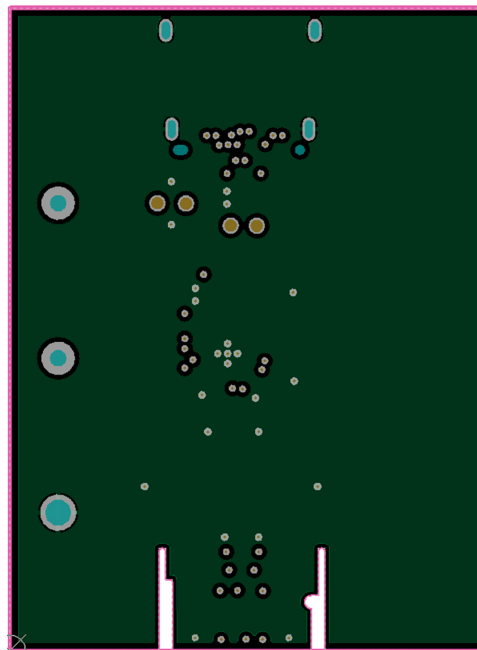
Figure 7. Ground Plane 2
