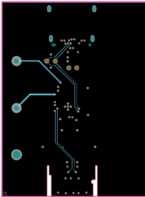
Figure 6. Midlayer 1
