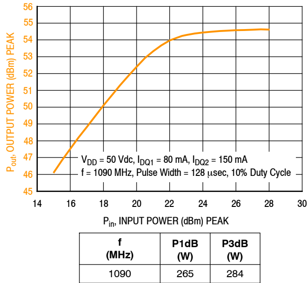
Figure 16. Output Power versus Input Power
