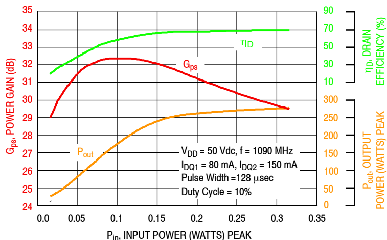
Figure 12. Power Gain, Drain Efficiency and Output Power versus Input Power
