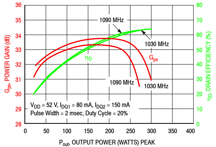
Figure 7. Power Gain and Drain Efficiency versus Output Power and Frequency — Long Pulse
