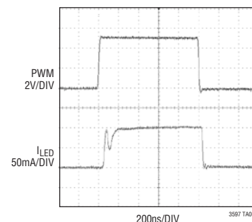
10,000:1 Dimming at 100Hz
