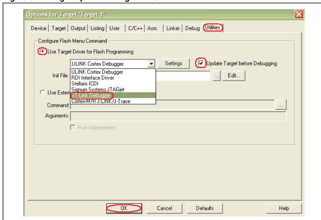
Figure 34. Target Options dialog box - Utilities tab
