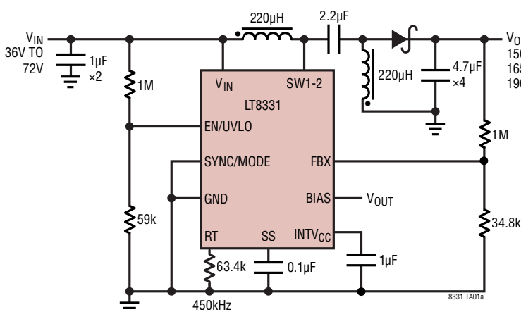
48V Output SEPIC Converter
