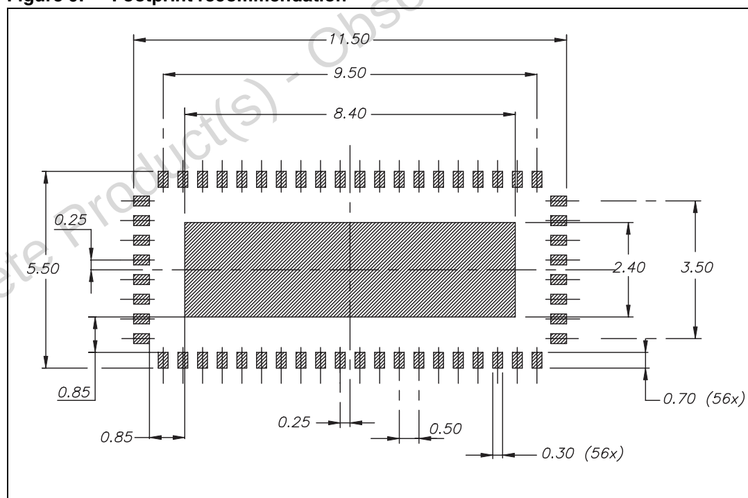
Figure 6. Footprint recommendation
