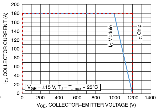
Figure 21. T1 & T4 RBSOA
