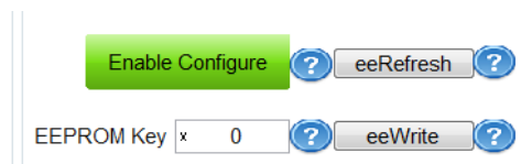
Figure 3. DRV10983 GUI
