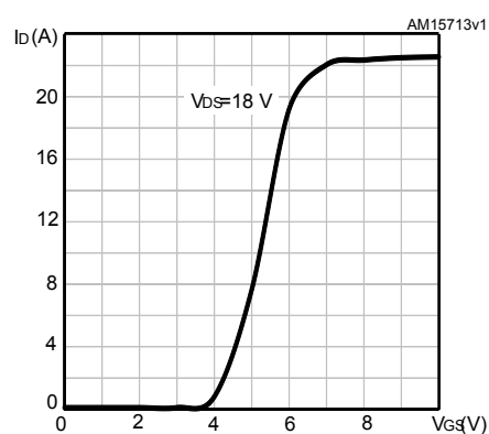
Figure 6. Transfer characteristics
