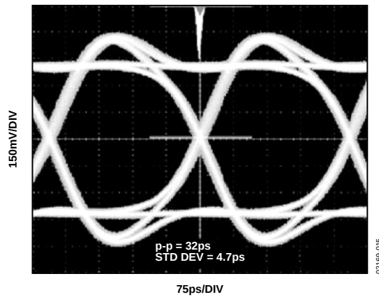
Figure 15. Crosstalk, 3.2 Gbps, PRBS 23, Attack Signal Is Off
