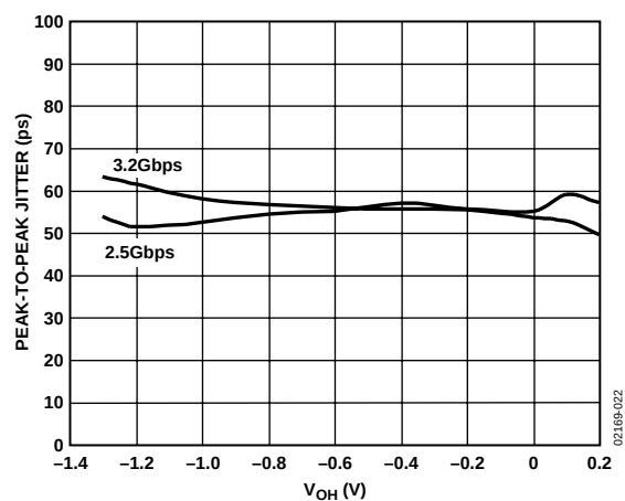
Figure 22. Jitter vs. V_{OH} , PRBS 23, Output Amplitude = 0.4 V Single-Ended
