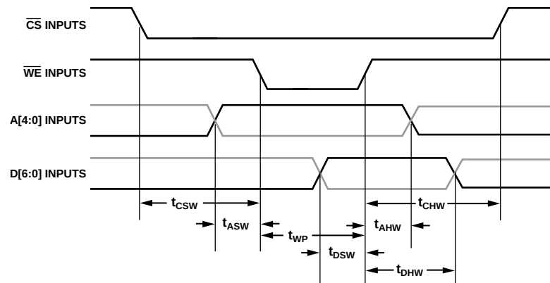
Figure 27. First Rank Write Cycle
