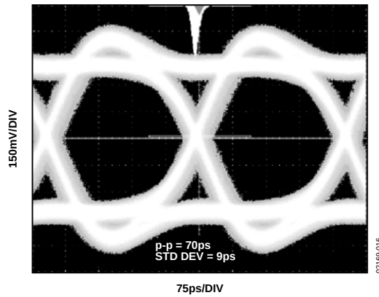
Figure 16. Crosstalk, 3.2 Gbps, PRBS 23, Attack Signal Is On
