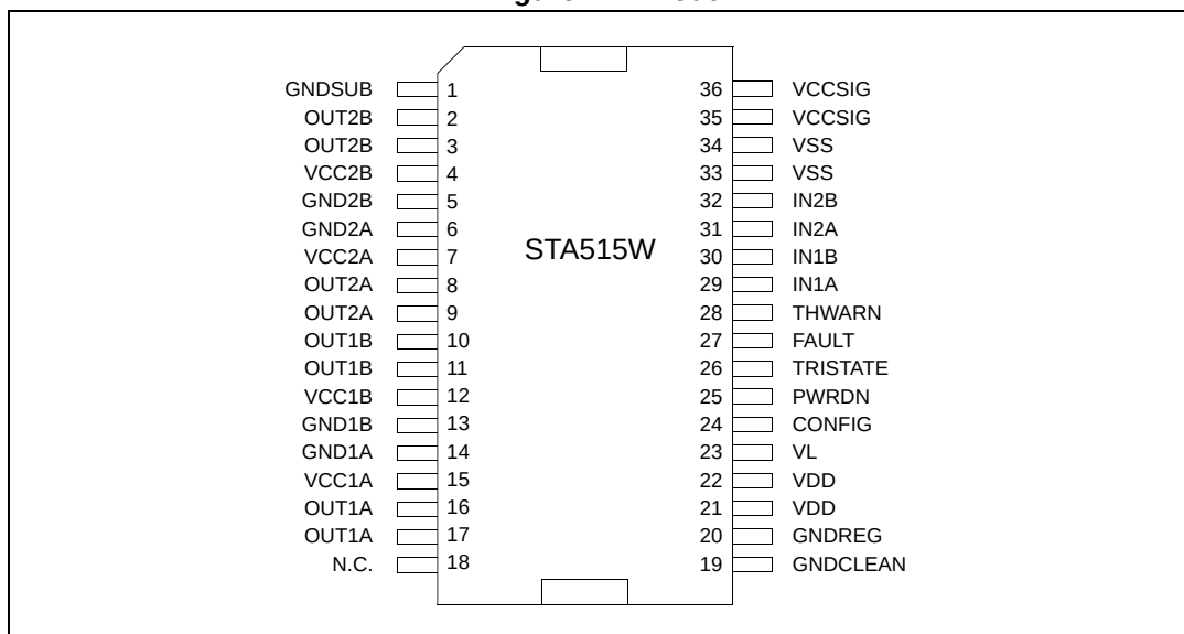
Figure 2. Pin out
