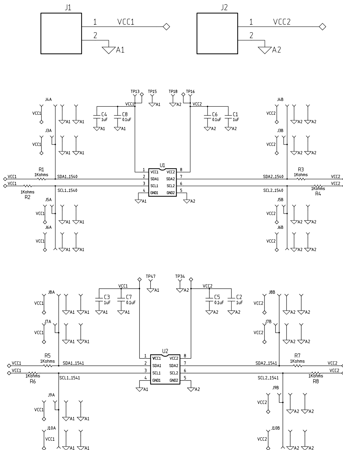
Figure 3. ISO154xEVM Schematic
