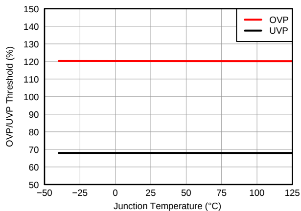
Figure 5. OVP/UVTP Threshold vs Junction Temperature
