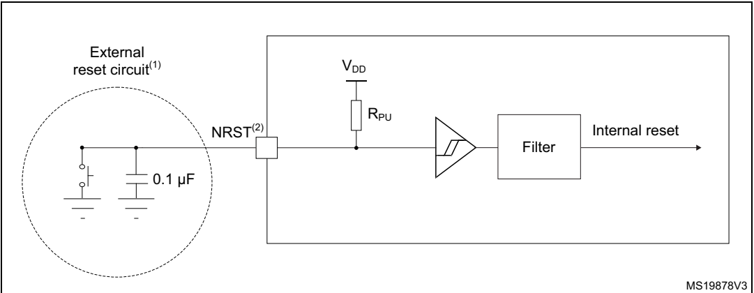
Figure 31. Recommended NRST pin protection
