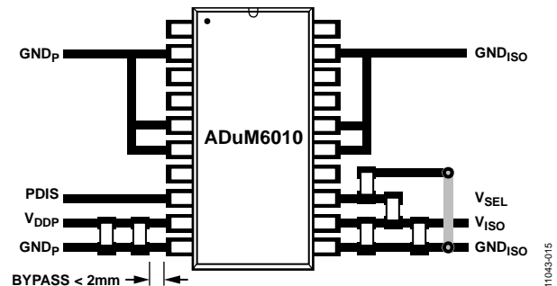
Figure 18. Recommended PCB Layout
