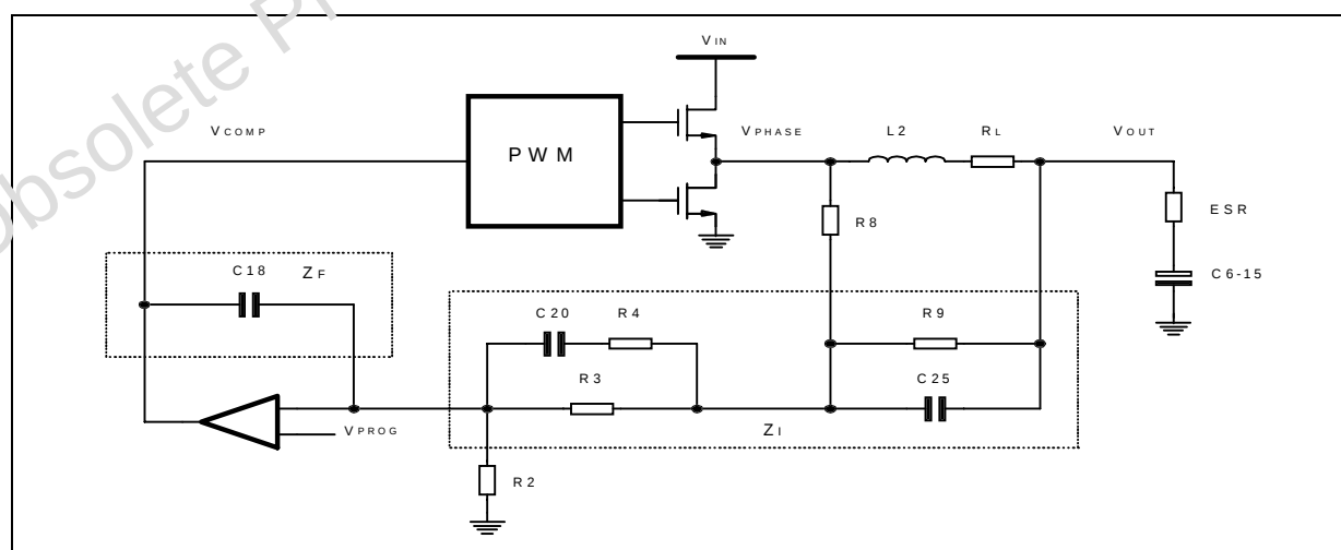
Figure 7. Compensation network
