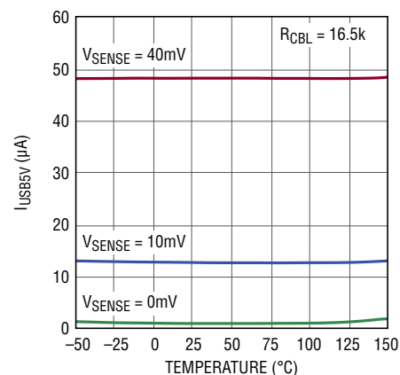
USB5V Current
