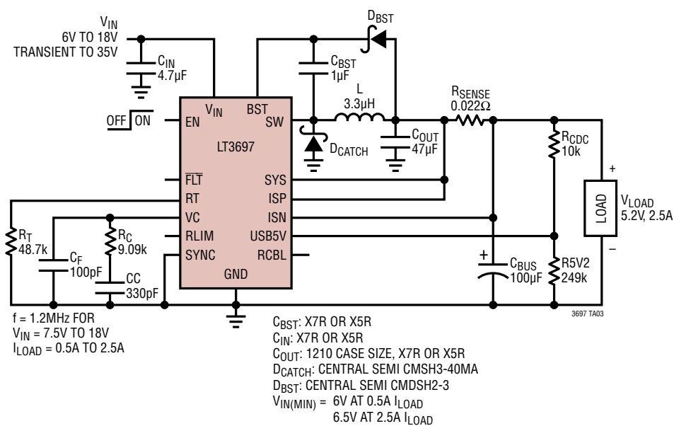
1.2MHz, 5.2V Step Down Converter with Output Current Limit
