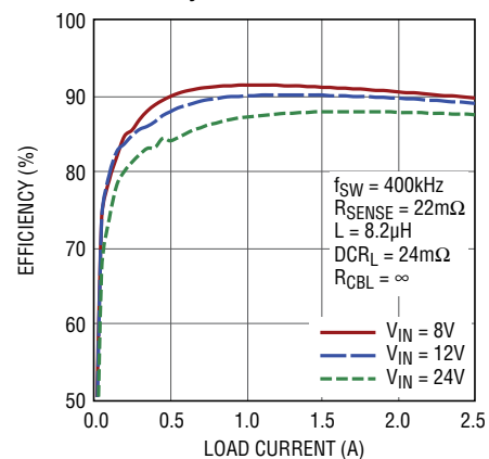
Efficiency at 400kHz
