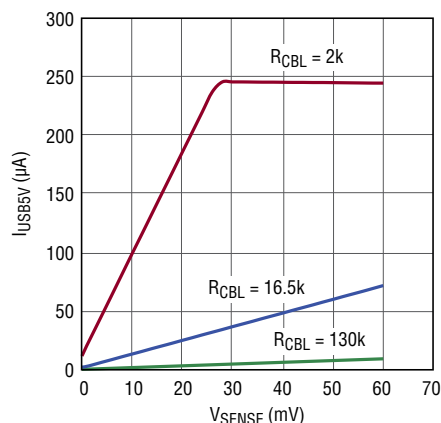
USB5V Current
