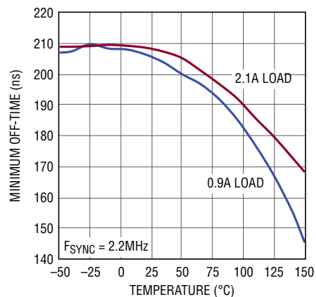
Minimum Off-Time in SYNC
