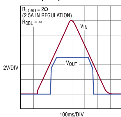
Start-Up/Dropout Performance
