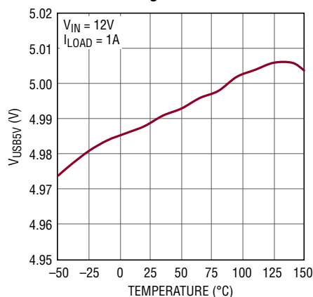
USB5V Voltage
