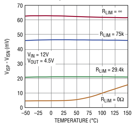
Sense Voltage ( V_{ISP} - V_{ISN} ) at 4.5V Output
