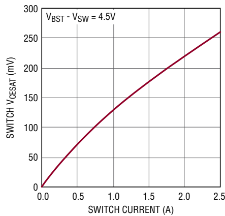
Switch V_{\text{CESAT}}
