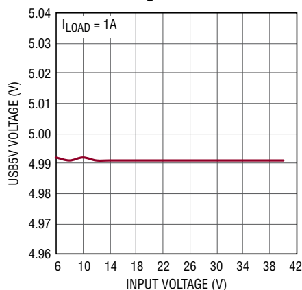
USB5V Voltage
