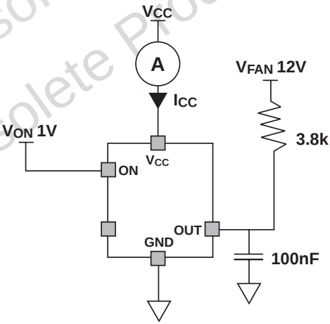
Fig. 5: I_{CC} versus V_{CC} test circuit (mode ON).
