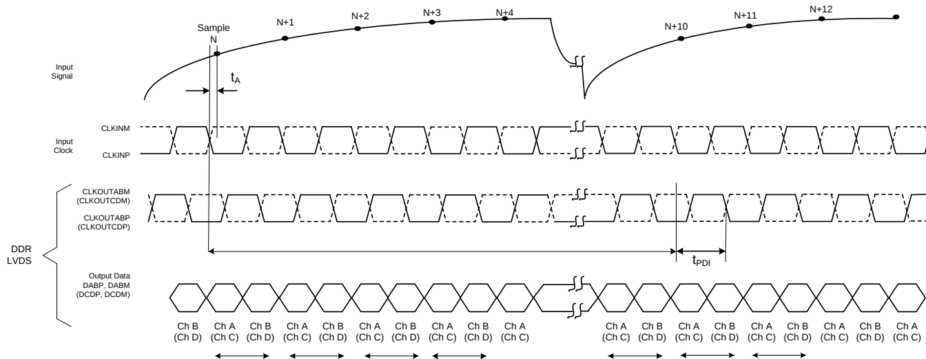
Figure 2. Latency Timing
