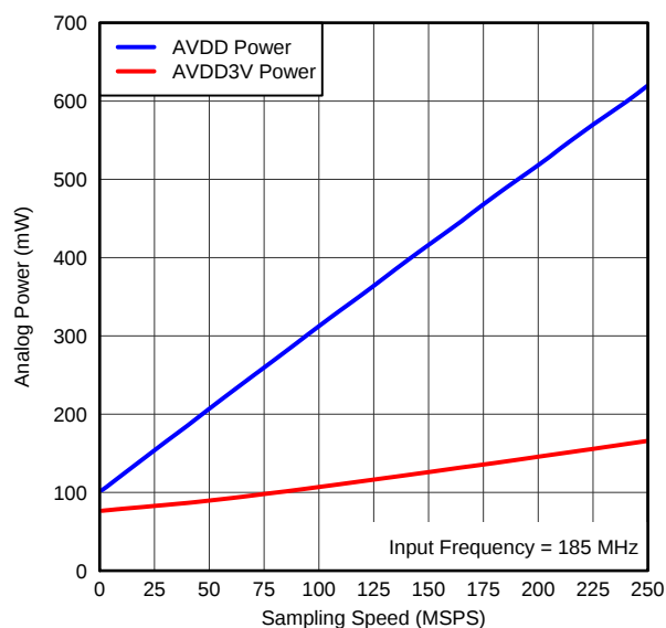
Figure 38. ANALOG POWER vs SAMPLING RATE
