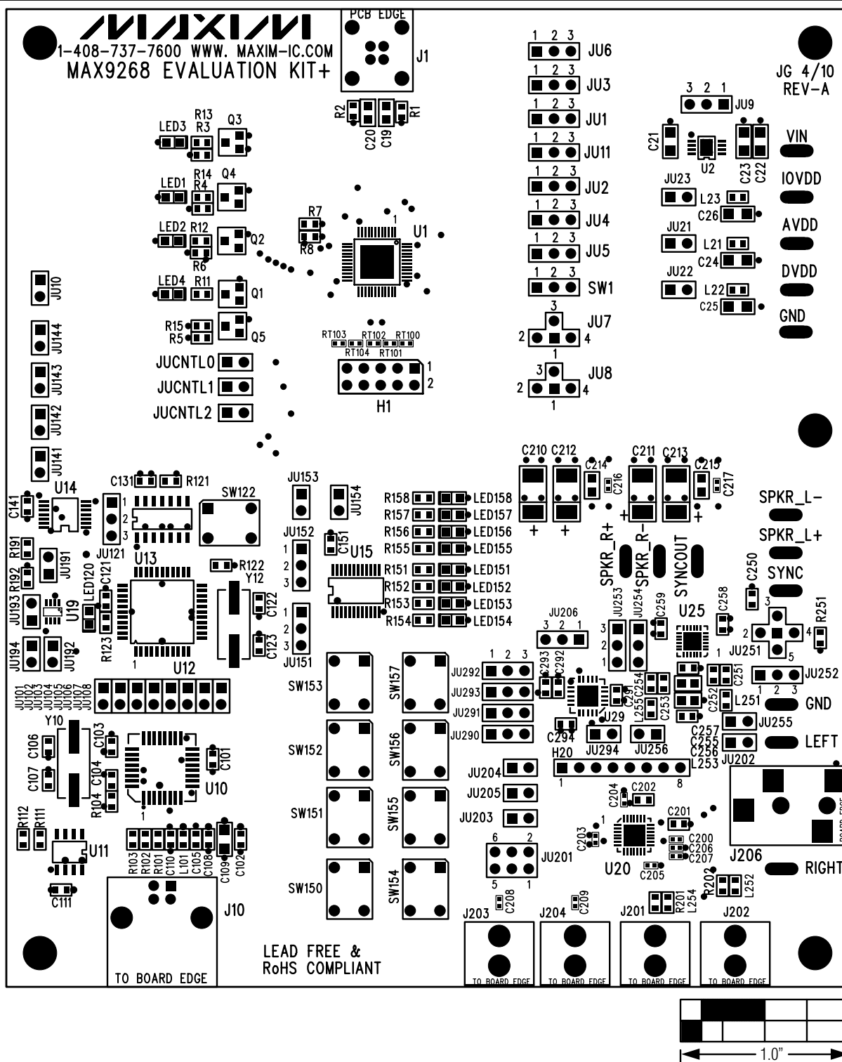
Figure 9. MAX9268 EV Kit Component Placement Guide—Component Side
