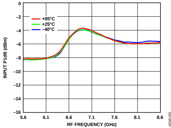
Figure 55. Input P1dB vs. RF Frequency over Temperatures, LO Power = 0 dBm
