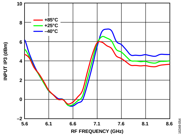
Figure 54. Input IP3 vs. RF Frequency over Temperatures, LO Power = 0 dBm
