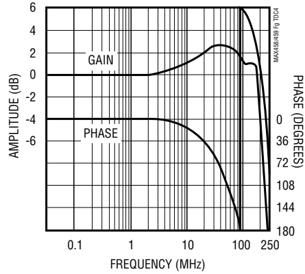
MAX458 GAIN vs. FREQUENCY
