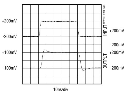
MAX458 SMALL-SIGNAL PULSE RESPONSE
