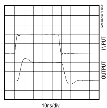
MAX459 SMALL-SIGNAL PULSE RESPONSE
