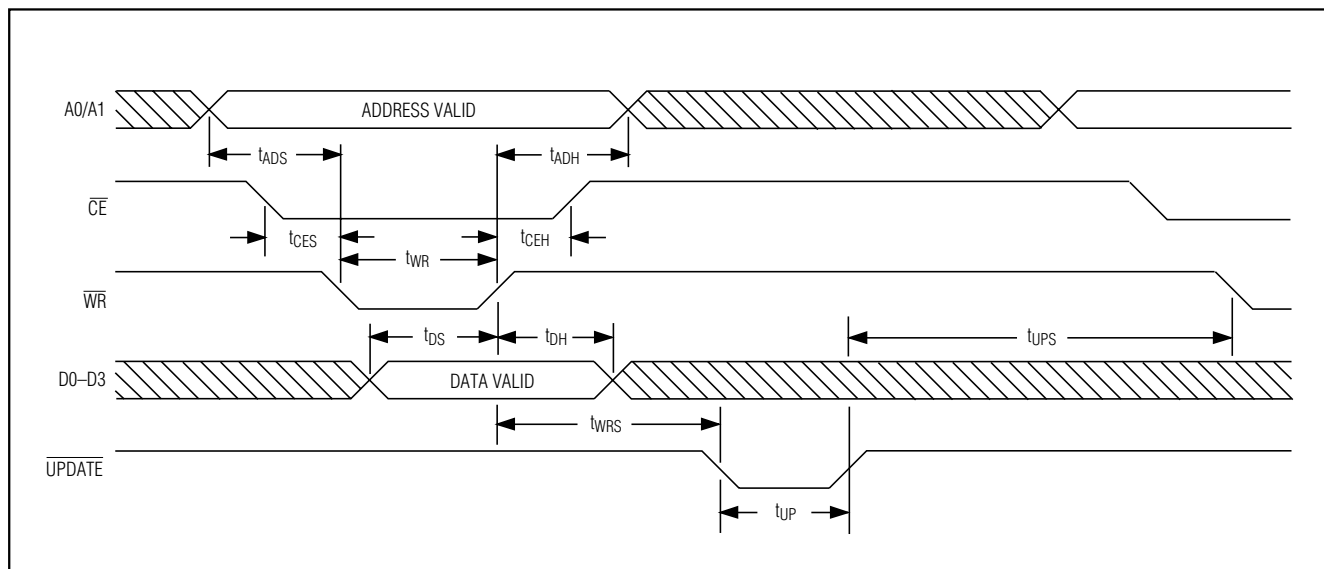
Figure 4. Parallel-Mode Timing
