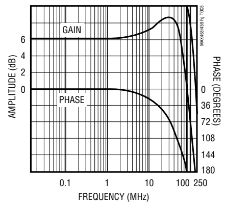
MAX459 GAIN vs. FREQUENCY
