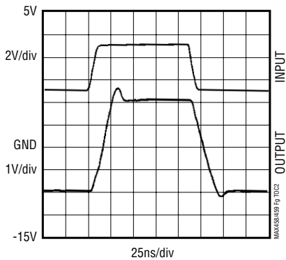
MAX458 LARGE-SIGNAL PULSE RESPONSE
