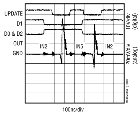
CHANNEL SWITCH TRANSIENT
