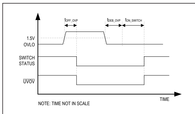
Figure 1. Overvoltage-Fault Timing Diagram
