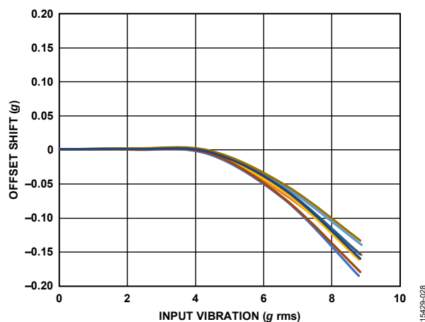
Figure 28. ADXL356 VRE, Z-Axis Offset from +1 g, \pm 10 g Range, Z-Axis Orientation = +1 g
