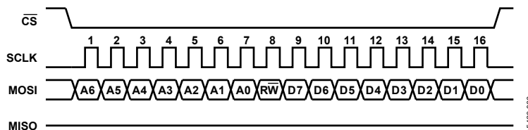
Figure 67. SPI Timing Diagram—Single-Byte Write
