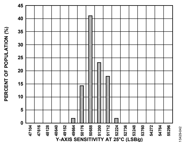
Figure 42. ADXL357 Sensitivity Histogram at 25°C, Y-Axis
