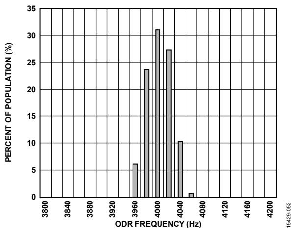
Figure 52. ADXL357 Output Data Rate (Internal Clock) Histogram
