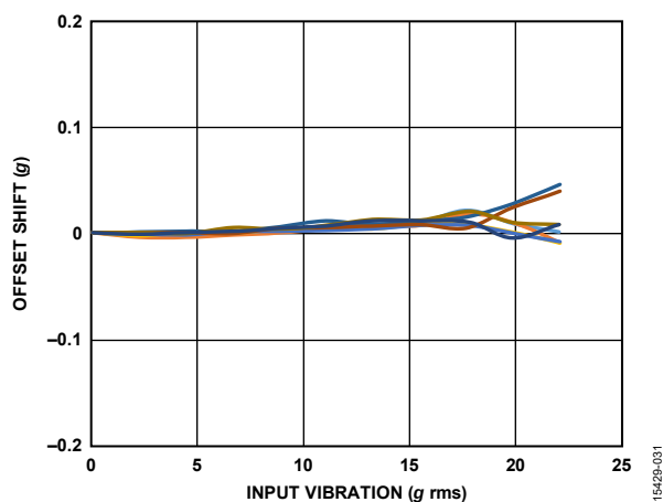
Figure 31. ADXL356 VRE, Z-Axis Offset from -1 g, \pm 40 g Range, Z-Axis Orientation = -1 g
