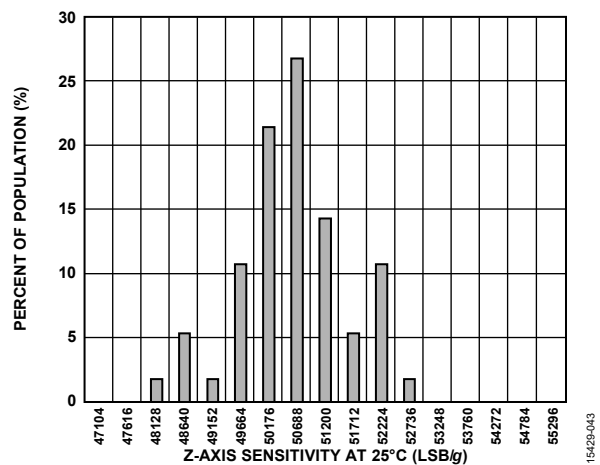
Figure 43. ADXL357 Sensitivity Histogram at 25°C, Z-Axis
