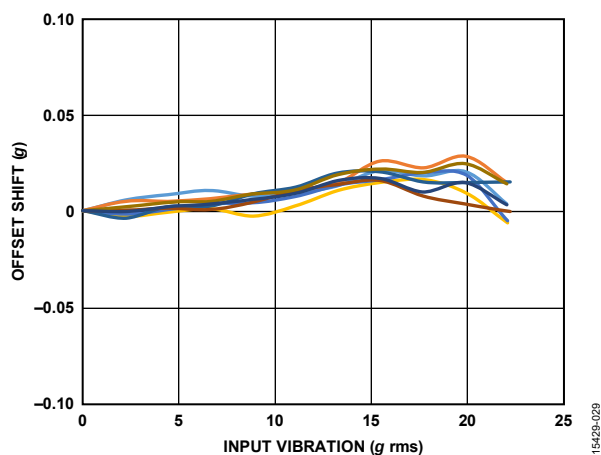
Figure 29. ADXL356 VRE, X-Axis Offset from -1 g, \pm 40 g Range, X-Axis Orientation = -1 g
