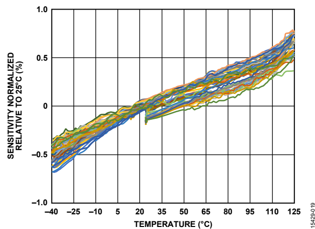
Figure 19. ADXL356 Sensitivity Normalized Relative to 25°C vs. Temperature, Z-Axis
