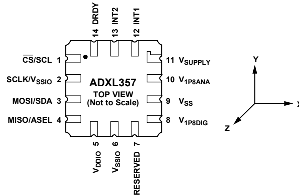
Figure 7. ADXL357 Pin Configuration (SPI/I²C)
