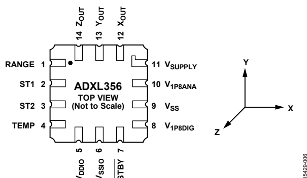
Figure 6. ADXL356 Pin Configuration
