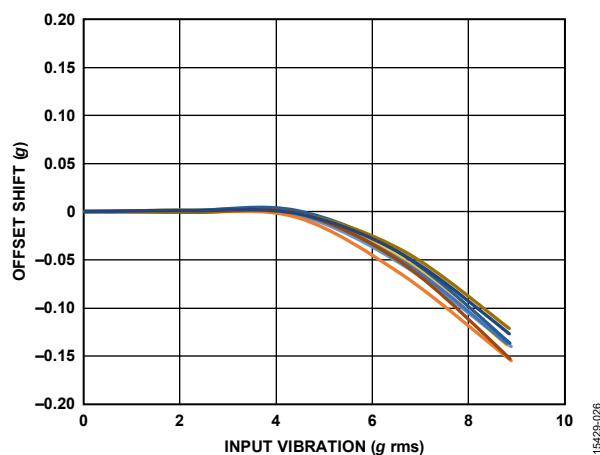
Figure 26. ADXL356 VRE, X-Axis Offset from +1 g, \pm 10 g Range, X-Axis Orientation = +1 g
