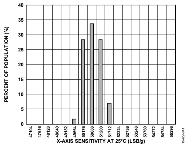
Figure 41. ADXL357 Sensitivity Histogram at 25°C, X-Axis
