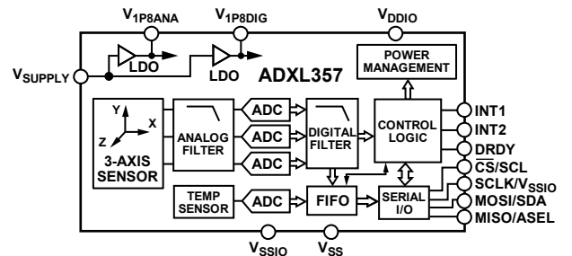
Figure 2. ADXL357
