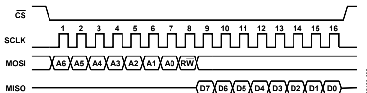
Figure 66. SPI Timing Diagram—Single-Byte Read
