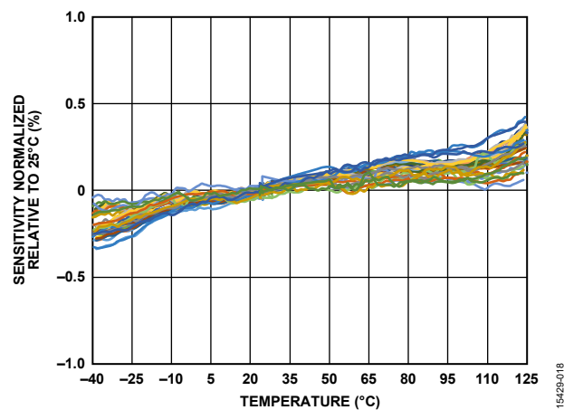
Figure 18. ADXL356 Sensitivity Normalized Relative to 25°C vs. Temperature, Y-Axis
