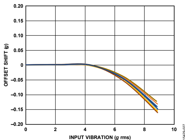
Figure 27. ADXL356 VRE, Y-Axis Offset from +1 g, \pm 10 g Range, Y-Axis Orientation = +1 g
