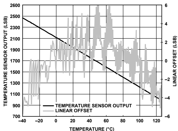
Figure 53. ADXL357 Temperature Sensor Output and Linear Offset vs. Temperature
