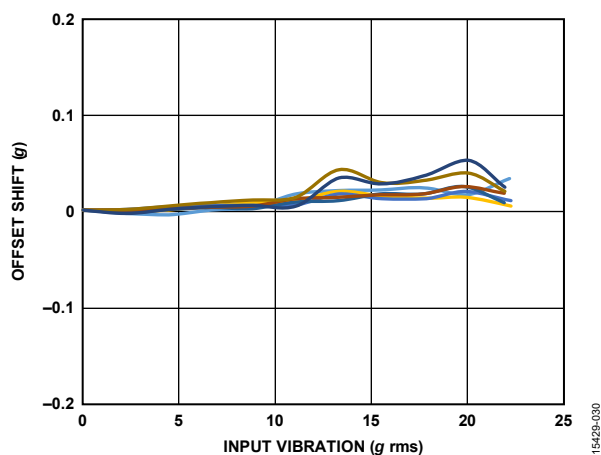
Figure 30. ADXL356 VRE, Y-Axis Offset from -1 g, \pm 40 g Range, Y-Axis Orientation = -1 g
